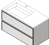
WD2214-0 W900xD460xH500mm
