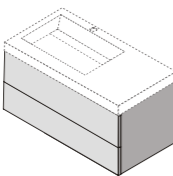
WD2113-0 W900xD460xH500mm
