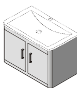
WD2069-0 W800xD460xH550mm
