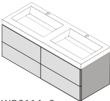
WD2114-0 W1200xD460xH500mm
