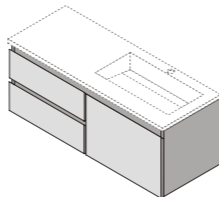
WD2216R-0 W1200xD460xH440mm
