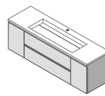
WD2208-0 W1600xD460xH500mm
