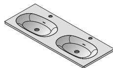
WD38360 W1200xD460xH130mm
