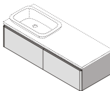
WD2805L-0 W1200xD460xH300mm
