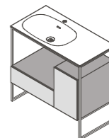
WD2701-0 W900xD480xH850mm
