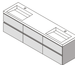
WD2926-0 W1800xD460xH500mm
